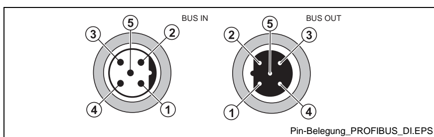
Fig. 4-18: PROFIBUS pin assignment (encoded according to M12 B)
