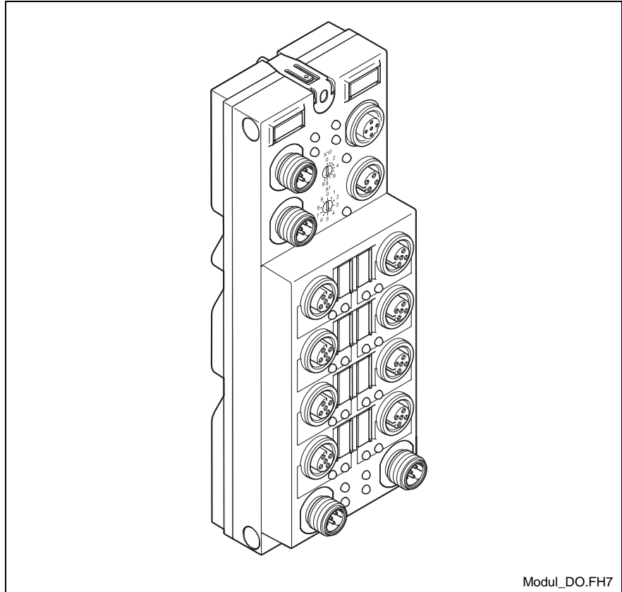
Fig. 6-1: RECO Fieldline device RF-FLS PB M12 DO 8 M12-2A
