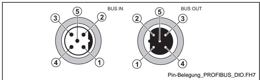
Fig. 5-23: PROFIBUS pin assignment (encoded according to M12 B)
