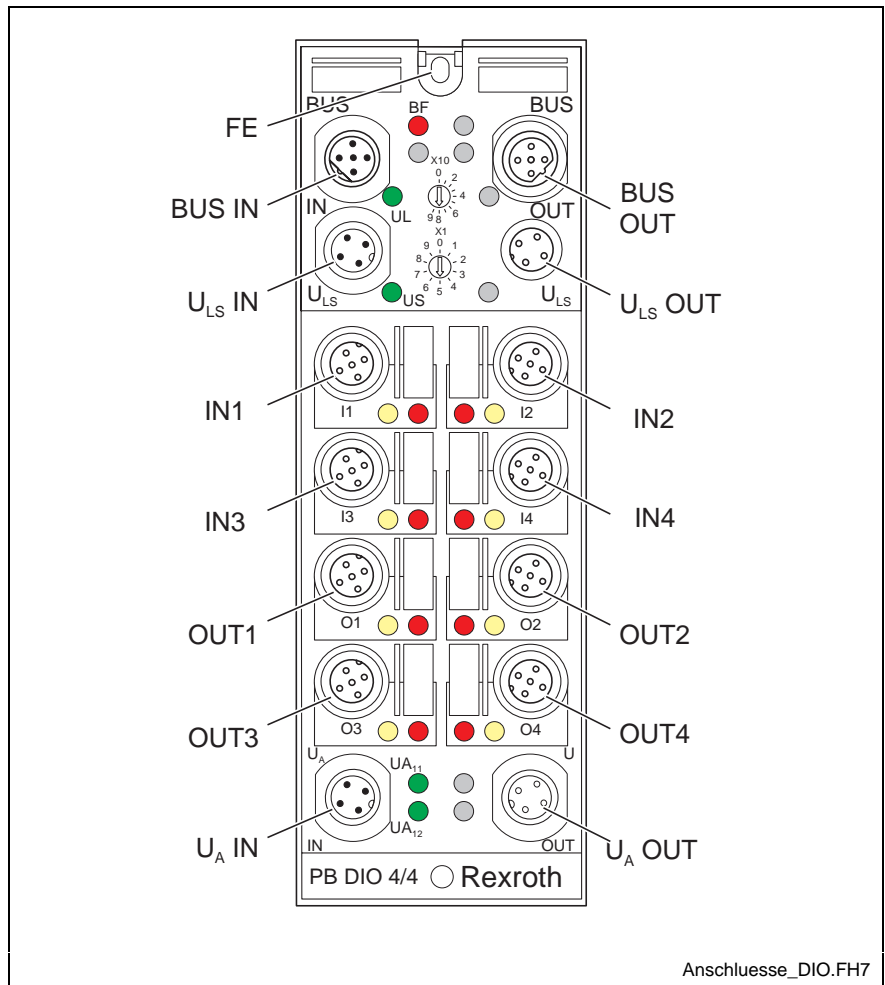
Fig. 5-21: Device connections RF-FLS PB M12 DIO 4/4 M12-2A
