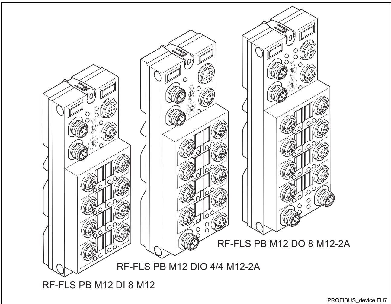
Fig. 1-1: PROFIBUS devices
