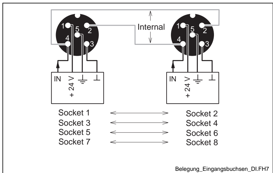
Fig. 4-24: Assignment of the input sockets
