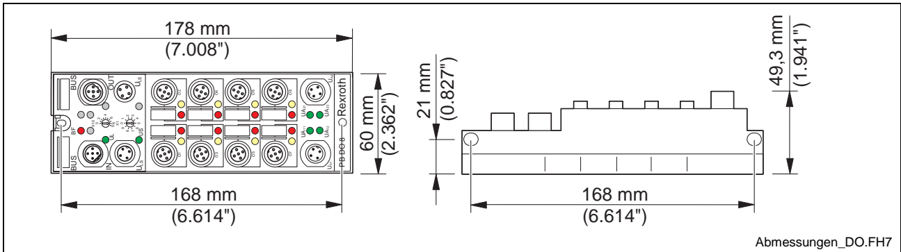
Fig. 6-4: Device Dimensions
