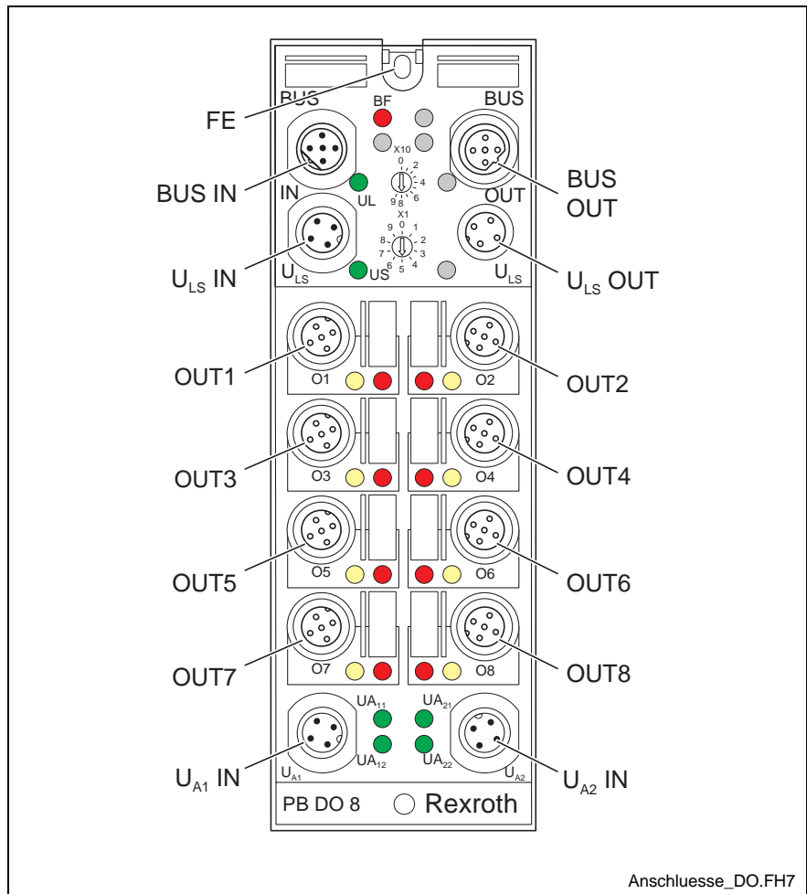
Fig. 6-17: Device connections RF-FLS PB M12 DO 8 M12-2A
