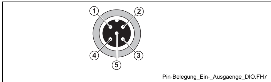
Fig. 5-29: Pin assignment of the inputs and outputs
