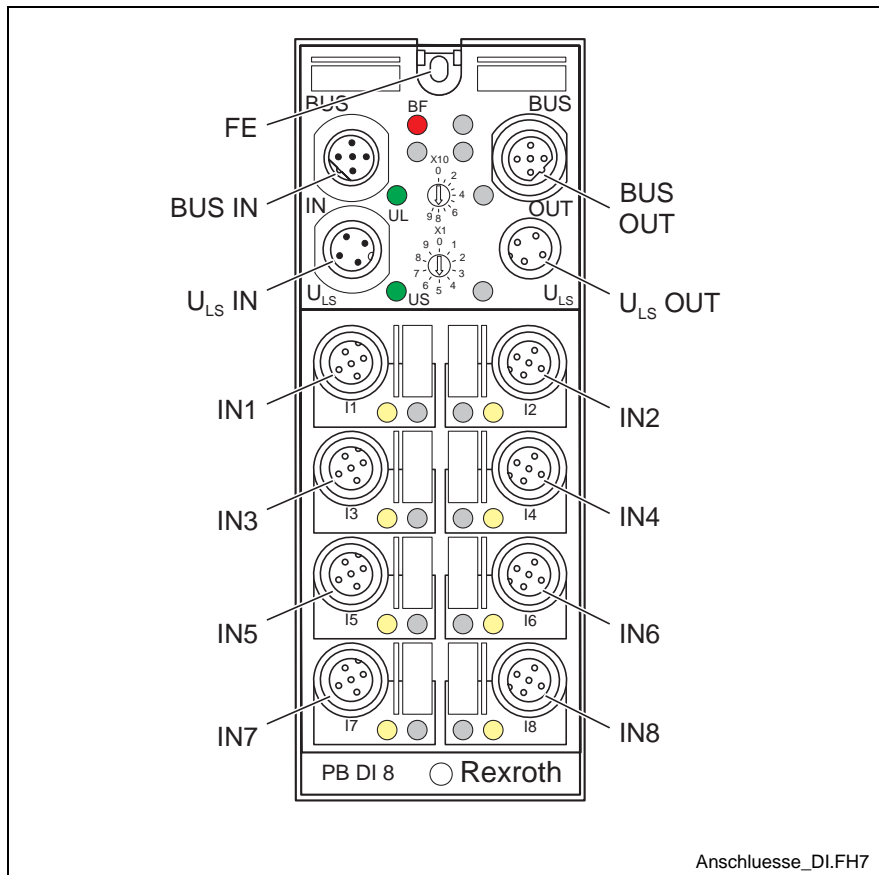
Fig. 4-16: Connections of the device
