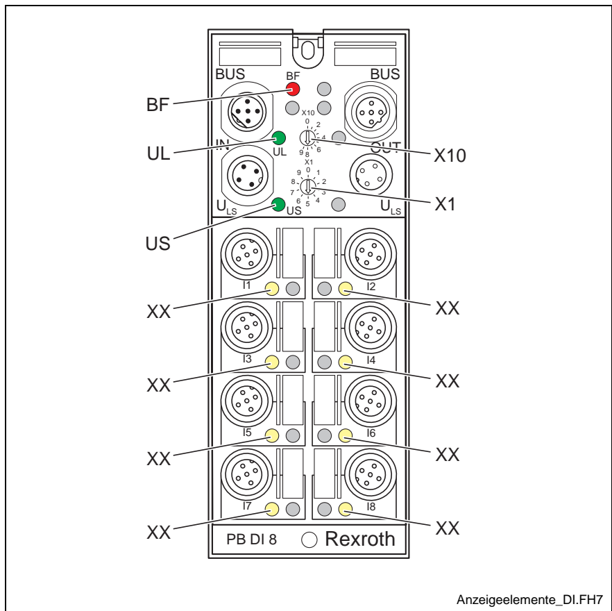
Fig. 4-2: Diagnostic and status indicators
