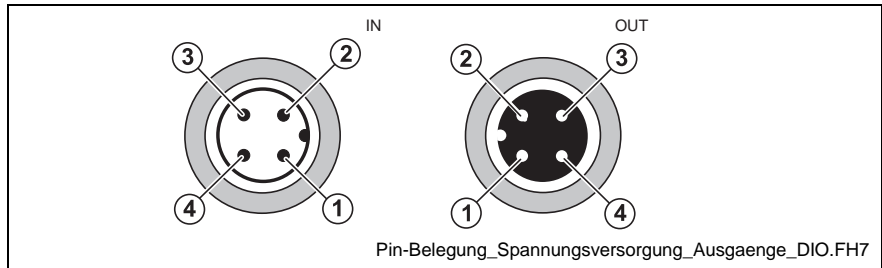
Fig. 5-27: Pin assignment of the voltage supply U_A of the outputs
