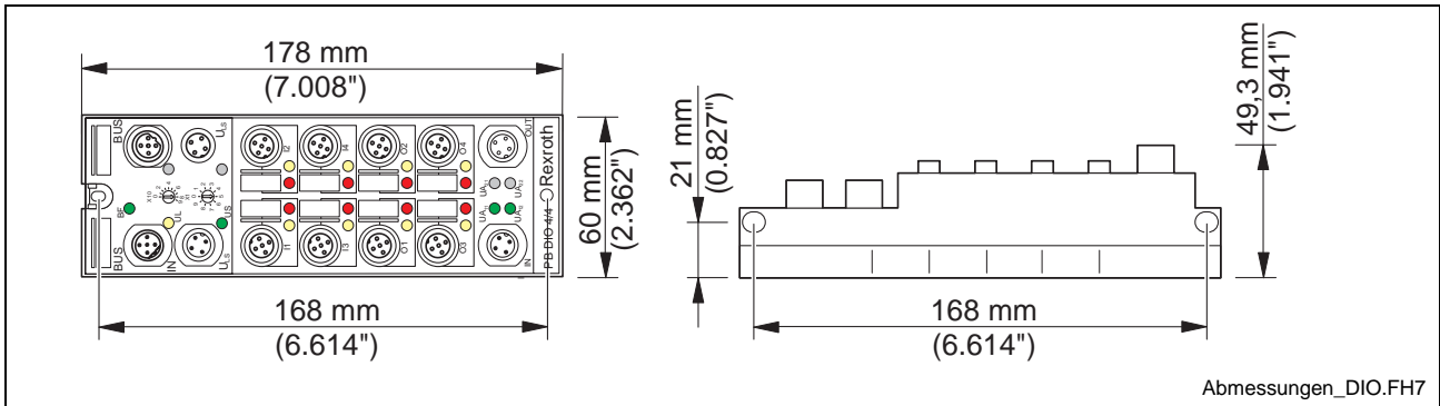
Fig. 5-4: Device dimensions
