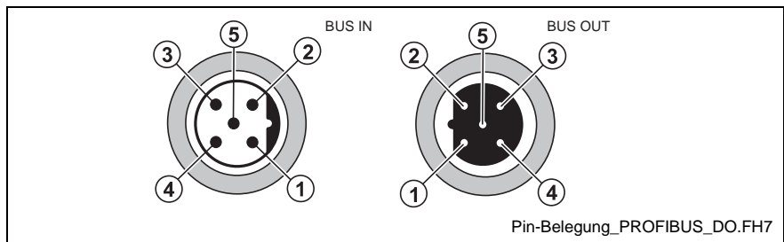
Fig. 6-19: PROFIBUS pin assignment (encoded according to M12 B)
