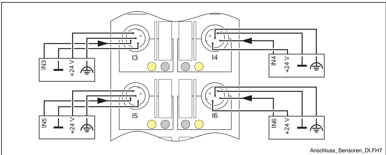
Fig. 4-27: Sensor connection example
