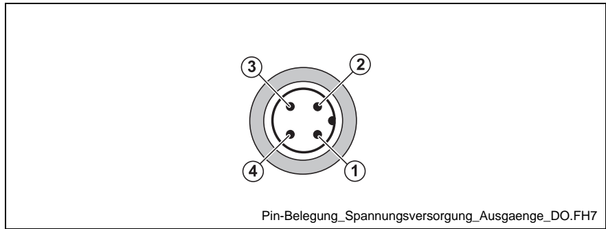
Fig. 6-23: Pin assignment of the voltage supply U_A of the outputs
