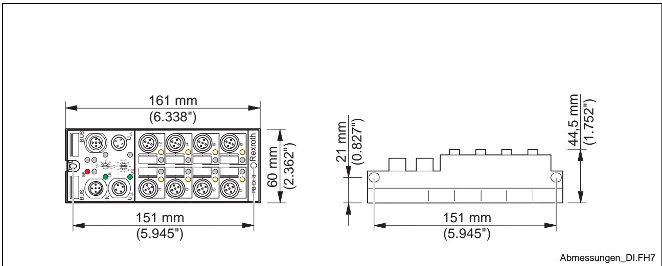
Fig. 4-4: Device dimensions
